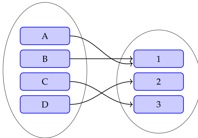
Figure 2.2: Each letter from the set containing A, B, C, D is related to exactly one output 1, 2, 3.
