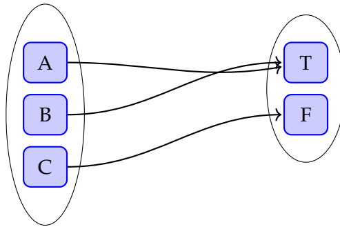
Figure 2.5: The interpretation function takes all the letters of the language of propositional logic (or those under consideration) and assigns them exactly one truth value: T or F.
